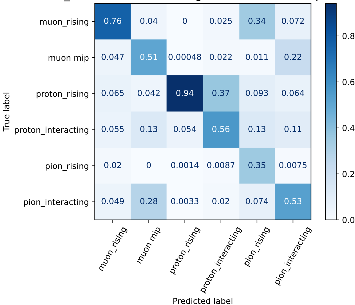
AdaBoost_purity confusion matrix n_estimators: 60 learning rate: 0.005 max depth: 5
