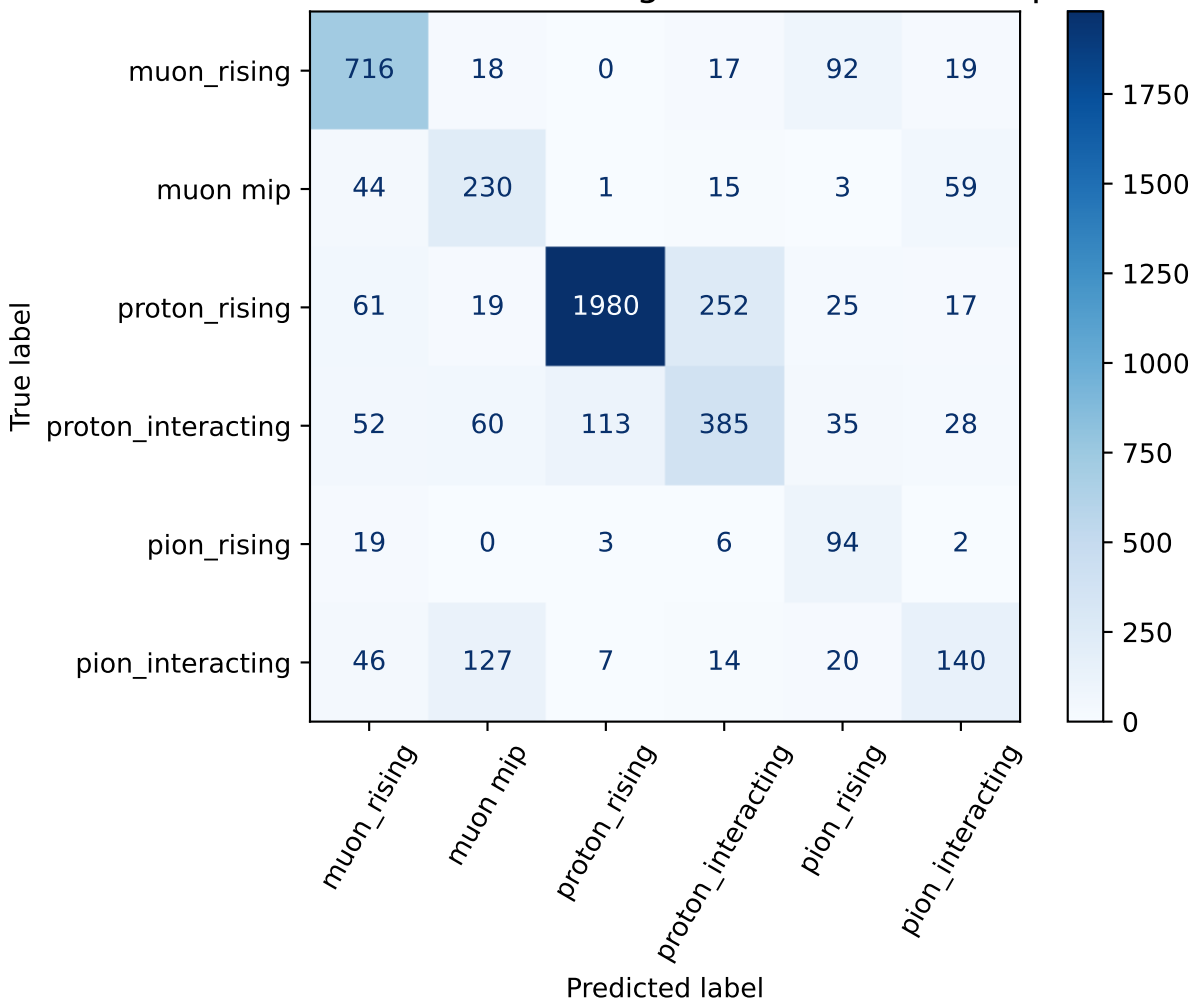
AdaBoost_confusion matrix n estimators: 60 learning rate: 0.005 max depth: 5
