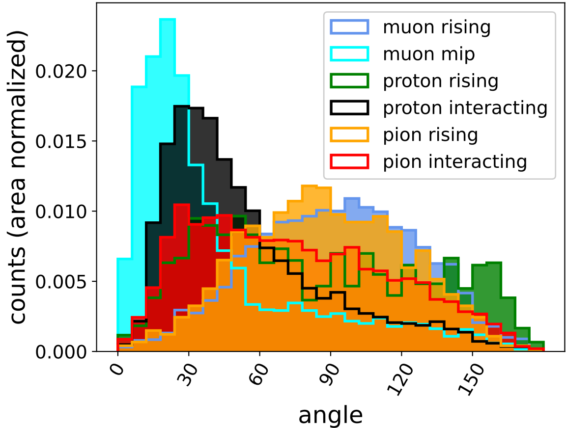
angle between mother start and daughter start directions
