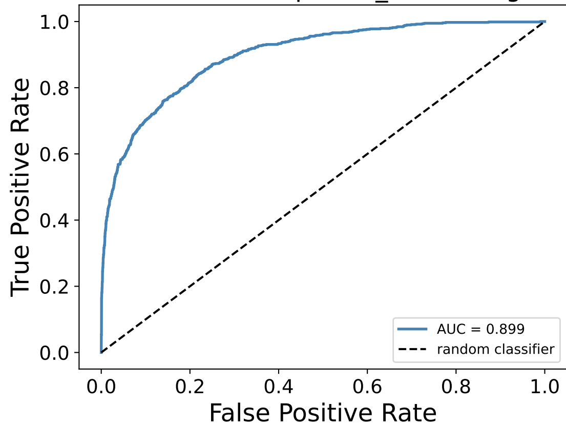
ROC curve — proton_interacting
