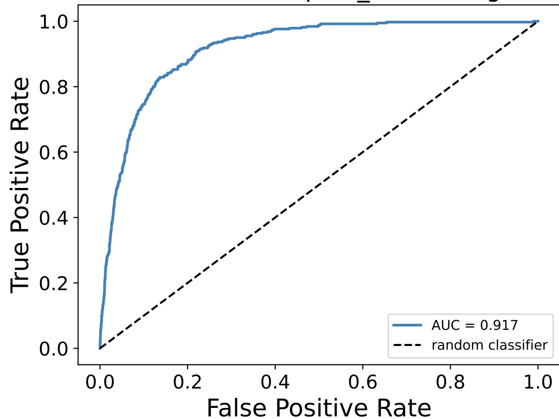
ROC curve — pion_interacting
