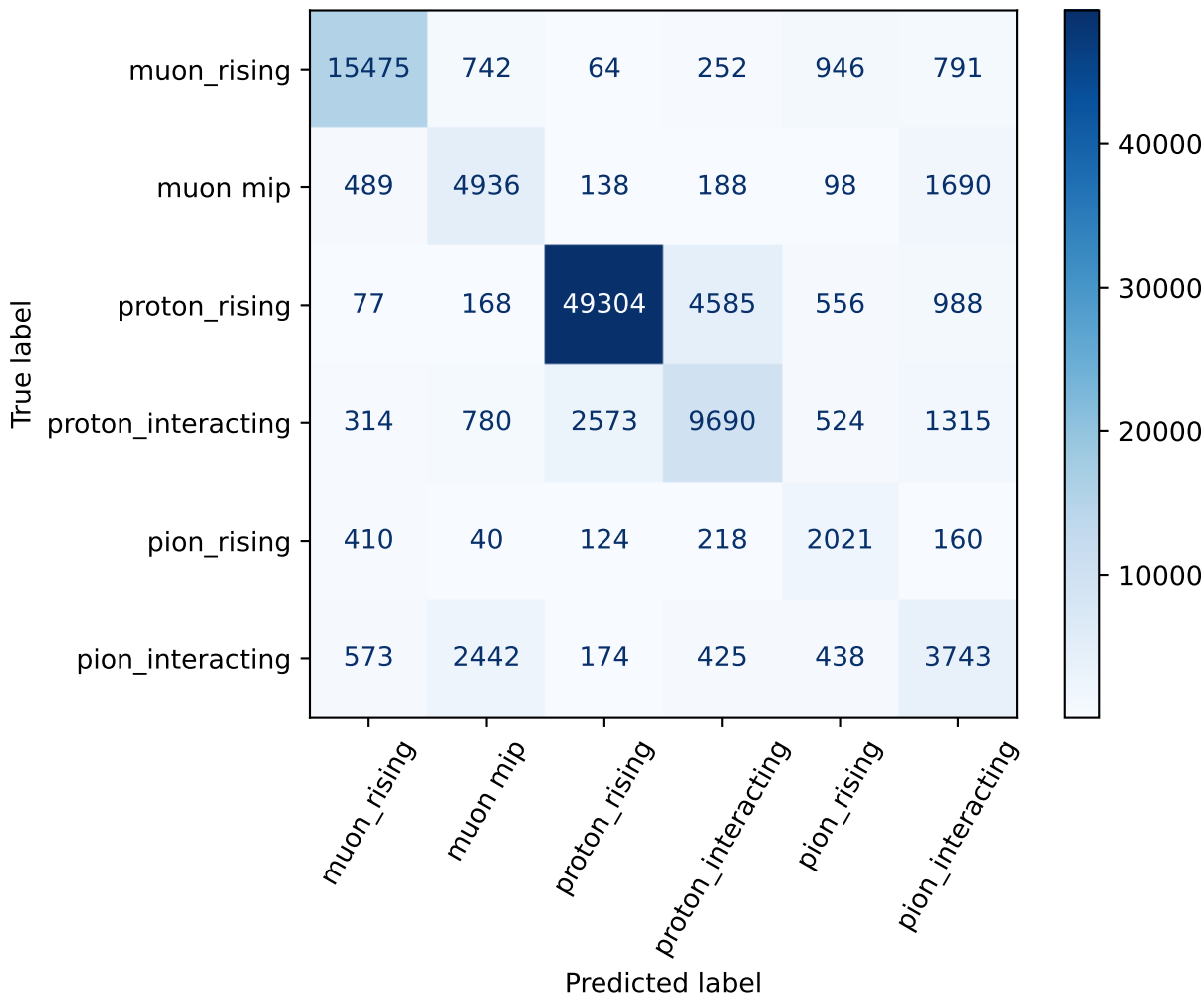
confusion matrix - 70% stat train ONLY COLL - test ONLY COLL
