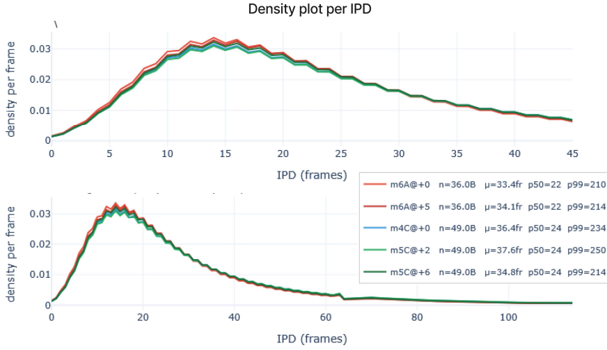
Figure 15: Density plot IPD
