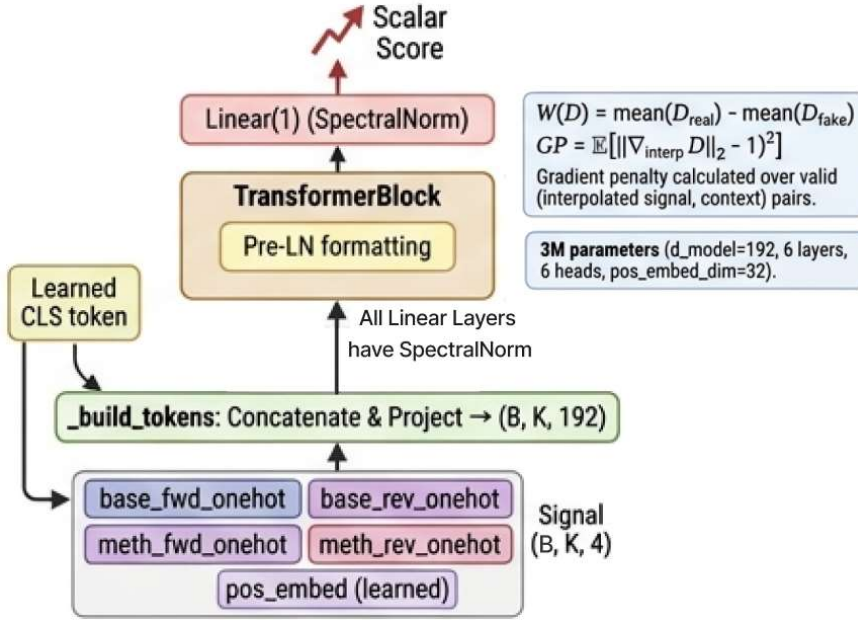
Figure 18: Critic's architecture
