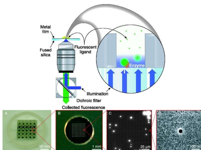
Figure 4: Zeromode waveguide representation [17]
