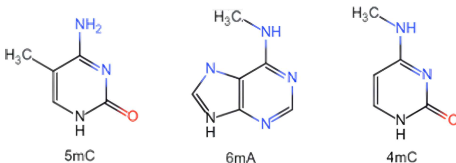
Figure 2: Representation of the main methylation types [15]
