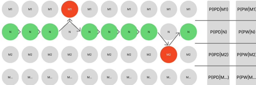
Figure 11: HMM simple representation for methylation
