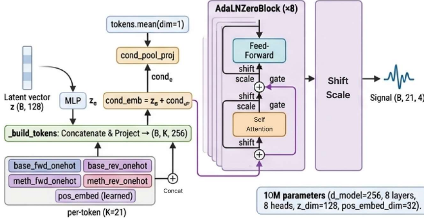
Figure 17: Generator architecture
