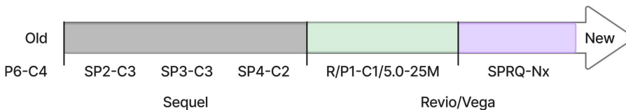
Figure 9: Non-exhaustive PacBio chemistry generation timeline
