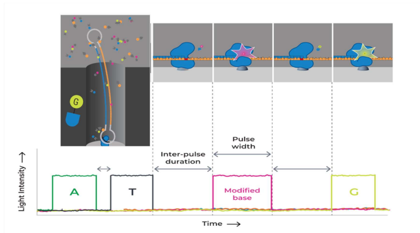
Figure 6: nucleotide incorporation kinetics in real time [19]
