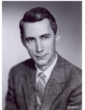
Claude Shannon
