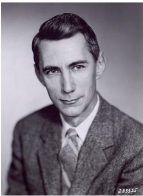
Claude Shannon
