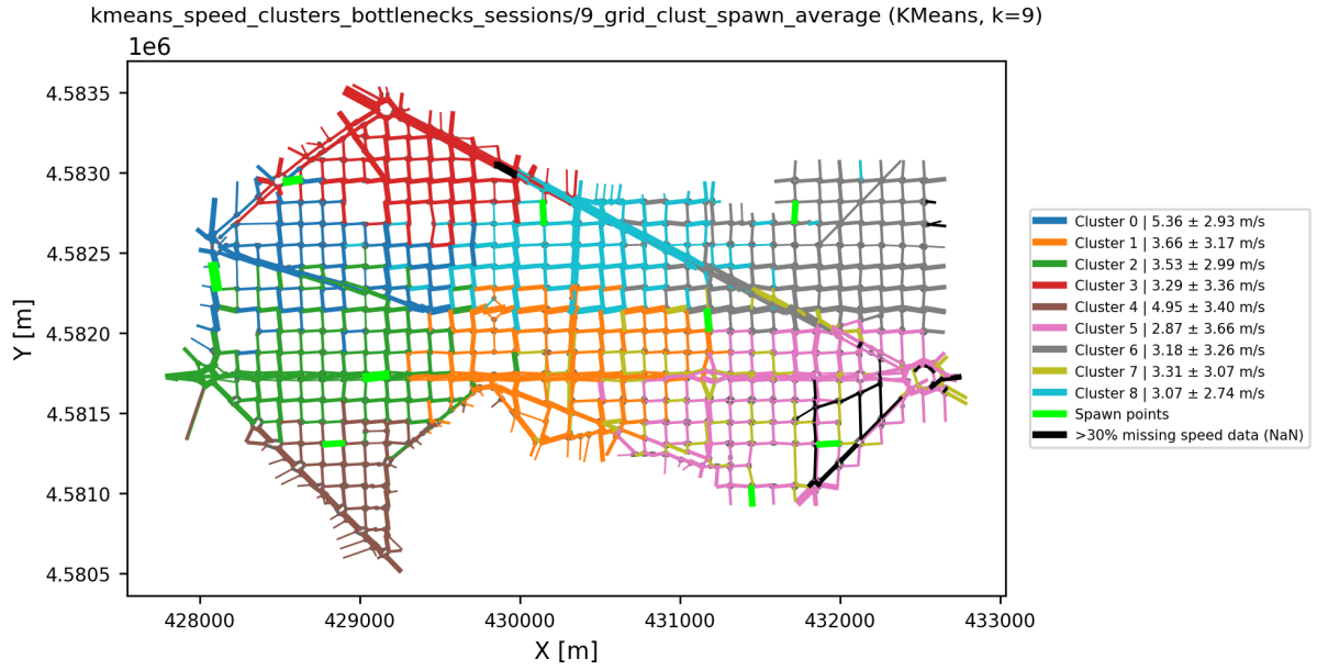
(b) K = 9
