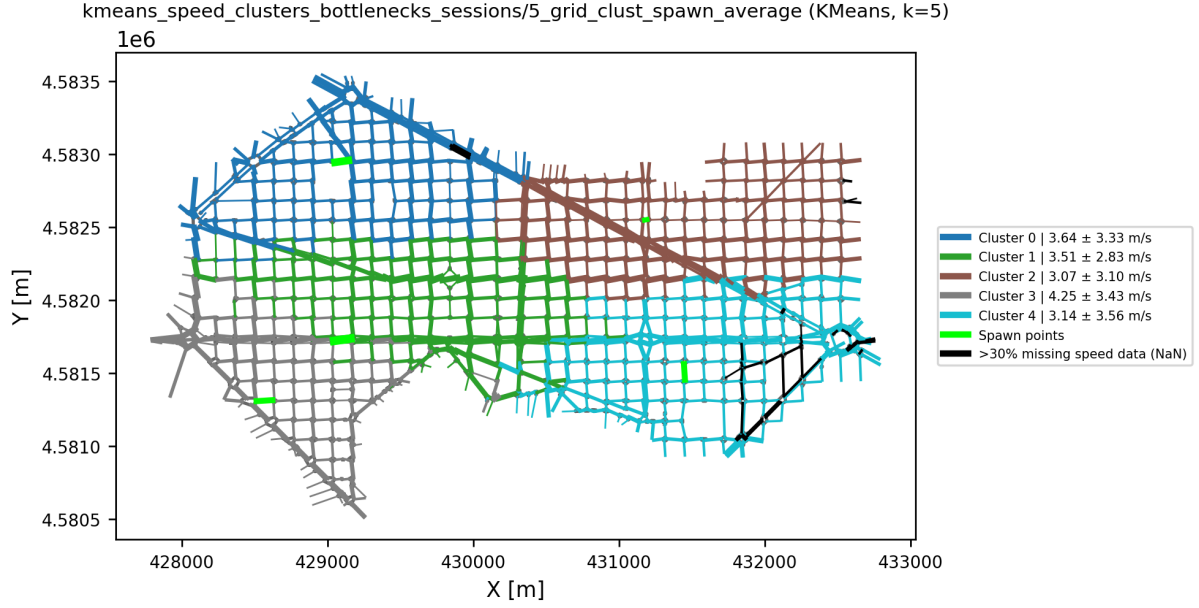
(a) K = 5
