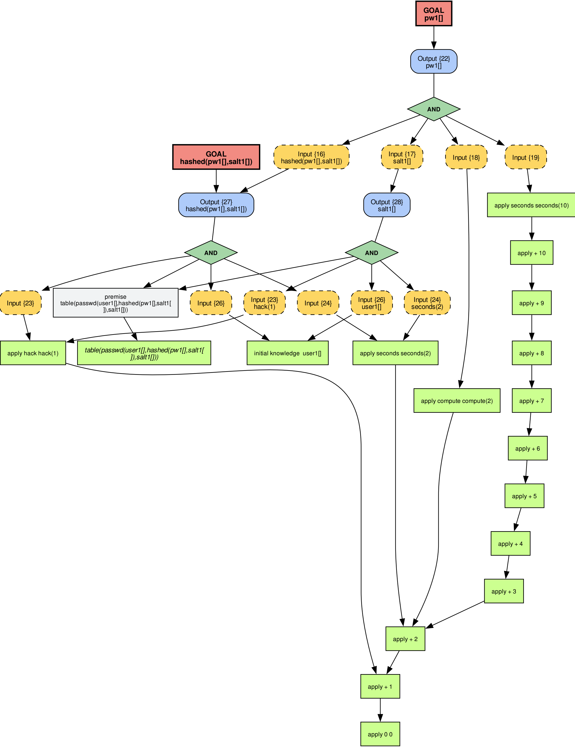
Master tree -- all goals (shared subtrees merged)
