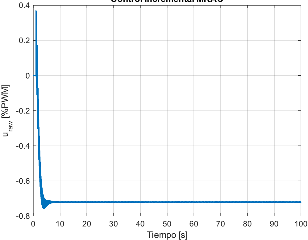
Control incremental MRAC
