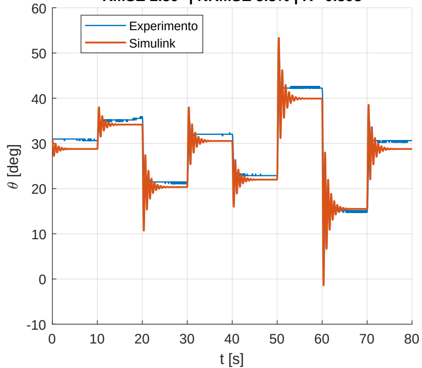
RMSE 2.59° | NRMSE 5.8% | R^2 0.898
