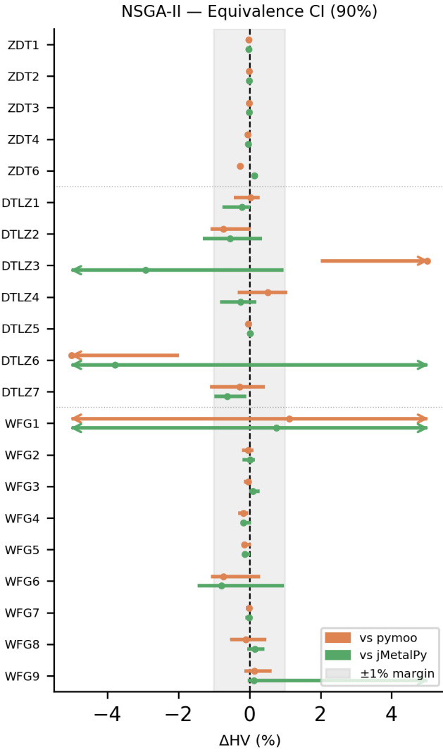
Fig. 2. NSGA-II. Per-problem paired bootstrap 90% confidence intervals for the relative normalized hypervolume difference \Delta = (HV_{VAMOS} - HV_{fw}) / HV_{fw} , reported in percent. The shaded band marks the \pm 1\% equivalence margin; intervals falling entirely within this band indicate statistical equivalence
