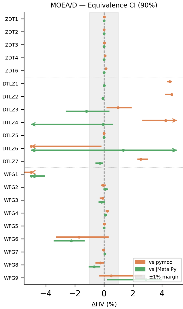
Fig. 5. MOEA/D. Per-problem paired bootstrap 90% confidence intervals for the relative normalized hypervolume difference \Delta = (HV_{VAMOS} - HV_{fw})/HV_{fw} , reported in percent. The shaded band marks the \pm 1\% equivalence margin; intervals falling entirely within this band indicate statistical equivalence
