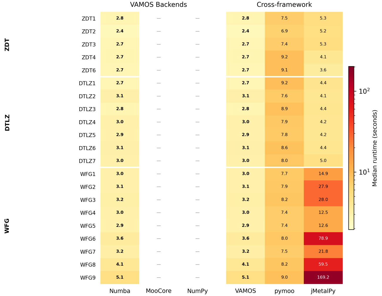
Fig. 3. Per-problem median runtime (seconds) for VAMOS backends (left) and cross-framework comparison (right). Color scale is logarithmic; bold values indicate the fastest in each row. Problems are grouped by family (ZDT, DTLZ, WFG).
