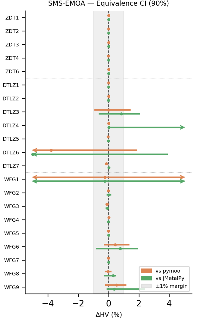
Fig. 4. SMS-EMOA. Per-problem paired bootstrap 90% confidence intervals for the relative normalized hypervolume difference \Delta = (HV_{VAMOS} - HV_{fw})/HV_{fw} , reported in percent. The shaded band marks the \pm 1\% equivalence margin; intervals falling entirely within this band indicate statistical equivalence
