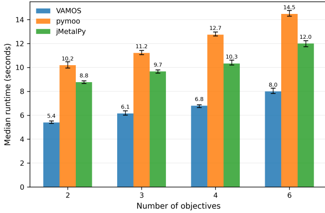
Fig. 5. Median runtime (seconds) of NSGA-II on ZCAT1-20 [36] by number of objectives. Bars show the median across per-problem medians (20 problems, 30 seeds each); error bars indicate the interquartile range. VAMOS maintains a consistent speedup advantage across all objective counts.
