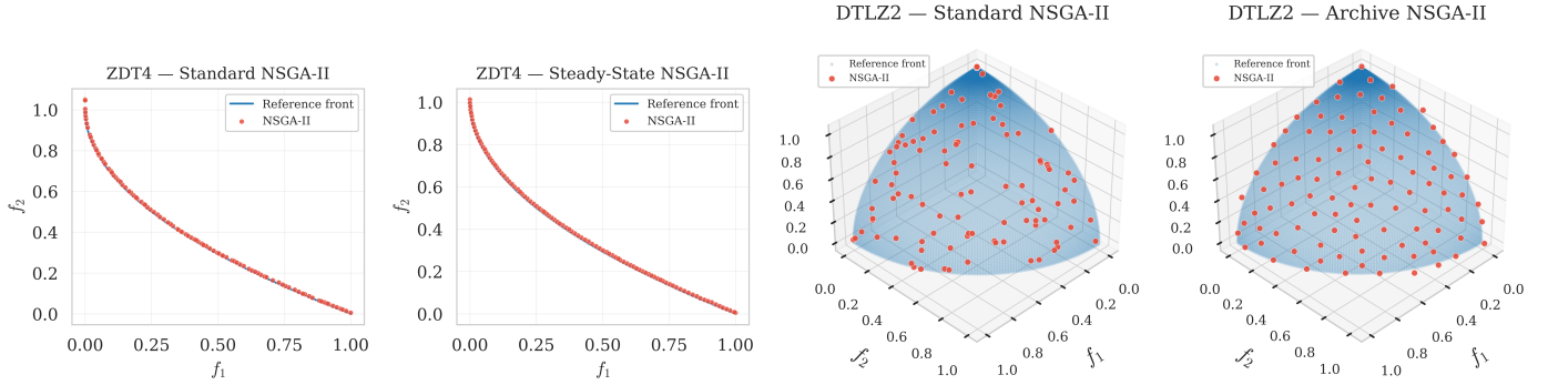
Fig. 6. Final non-dominated sets produced by NSGA-II variants on ZDT4 (left pair, 2-objective) and DTLZ2 (right pair, 3-objective), overlaid with the reference Pareto front. From left to right: (a) standard generational NSGA-II on ZDT4, (b) steady-state NSGA-II on ZDT4, (c) standard NSGA-II on DTLZ2, and (d) NSGA-II with unbounded external archive on DTLZ2. Both variants produce a more uniformly distributed approximation of the Pareto front.
