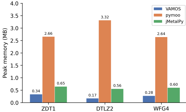
Fig. 7. Peak memory footprint (MB) during NSGA-II optimization on three representative problems (50,000 evaluations, median of 5 seeds). VAMOS consistently uses less memory than both pymoo and jMetalPy across all problem families.
