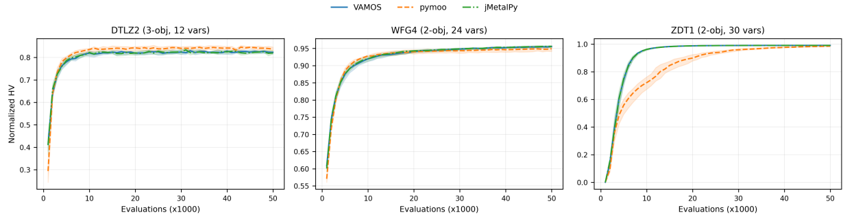
Fig. 8. Convergence of normalized hypervolume over 50,000 evaluations for VAMOS (Numba) and pymoo on DTLZ2 (3 objectives, 12 variables) and ZDT1 (2 objectives, 30 variables). Solid/dashed lines show median HV across 30 seeds; shaded regions indicate the interquartile range. Both frameworks follow nearly identical convergence trajectories, confirming that the semantic alignment protocol produces equivalent algorithmic behavior.
