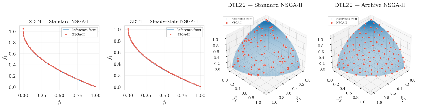
Fig. 6. Final non-dominated sets produced by NSGA-II variants on ZDT4 (left pair, 2-objective) and DTLZ2 (right pair, 3-objective), overlaid with the reference Pareto front. From left to right: (a) standard generational NSGA-II on ZDT4, (b) steady-state NSGA-II on ZDT4, (c) standard NSGA-II on DTLZ2, and (d) NSGA-II with unbounded external archive on DTLZ2. Both variants produce a more uniformly distributed approximation of the Pareto front.
