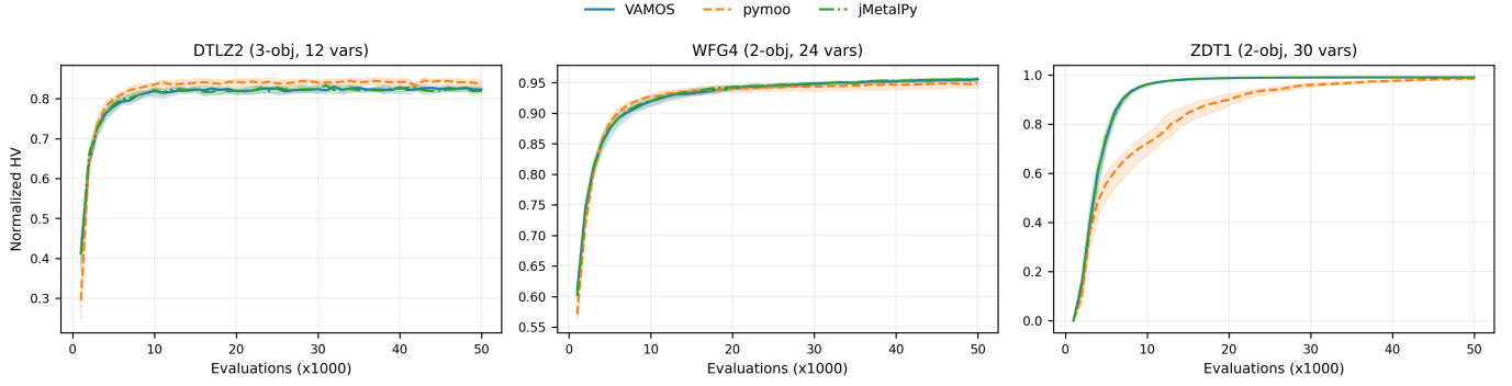
Fig. 1. Convergence of normalized hypervolume over 50,000 evaluations for VAMOS (Numba), pymoo , and jMetalPy on DTLZ2 (3 objectives, 12 variables), WFG4 (2 objectives, 24 variables), and ZDT1 (2 objectives, 30 variables). Solid/dashed lines show median hypervolume values across 30 seeds; shaded regions indicate the interquartile range. All three frameworks follow nearly identical convergence trajectories, confirming that the semantic alignment protocol produces equivalent algorithmic behavior.
