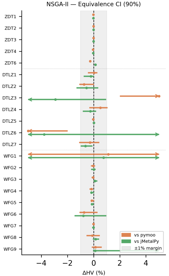
Fig. 3. NSGA-II. Per-problem paired bootstrap 90% confidence intervals for the relative normalized hypervolume difference \Delta = (HV_{\text{VAMOS}} - HV_{\text{fw}}) / HV_{\text{fw}} , reported in percent. The shaded band marks the \pm 1\% equivalence margin; intervals falling entirely within this band indicate statistical equivalence
