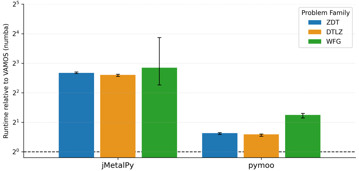
Fig. 7. Runtime of each framework relative to VAMOS (Numba) for generational NSGA-II, grouped by problem family (log 2 scale). Bars above the dashed parity line ( 2^0 = 1 ) indicate that the competitor is slower. Error bars show variability across per-problem medians within each family. All runs use 50,000 evaluations and 30 seeds.
