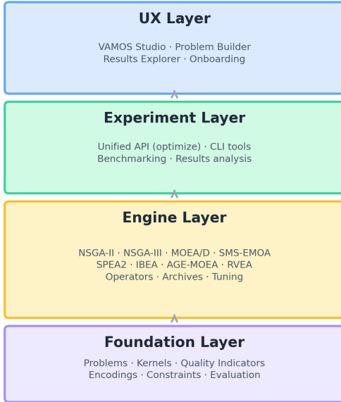
Fig. 1. VAMOS four-layer architecture.
