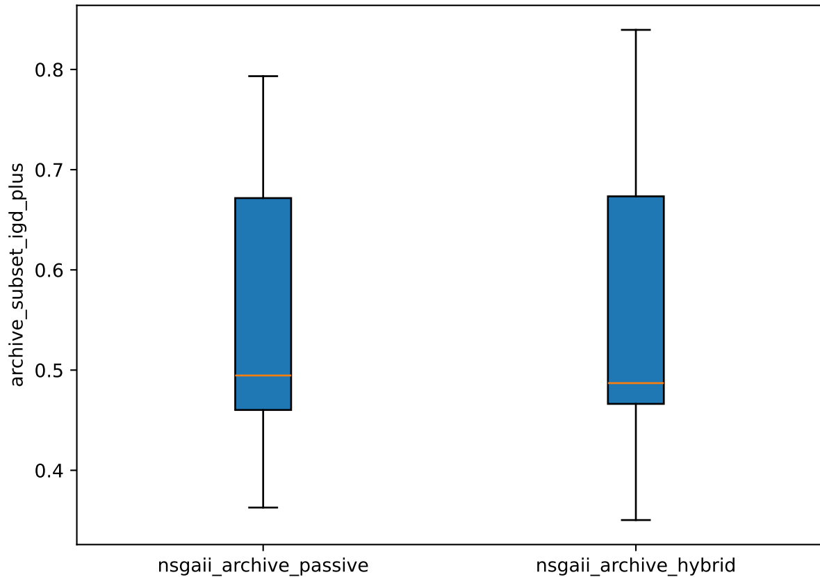
archive_subset_igd_plus | wfg1
