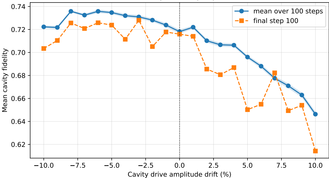
Post-training sensitivity to cavity-drive amplitude 1000 trajectories per point
