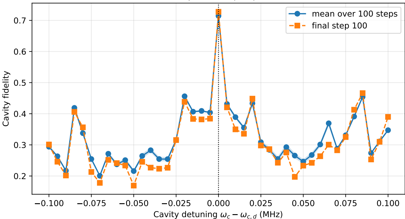
Post-training sensitivity to cavity-frequency drift 50 trajectories per point
