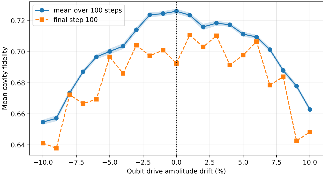
Post-training sensitivity to qubit-drive amplitude 1000 trajectories per point
