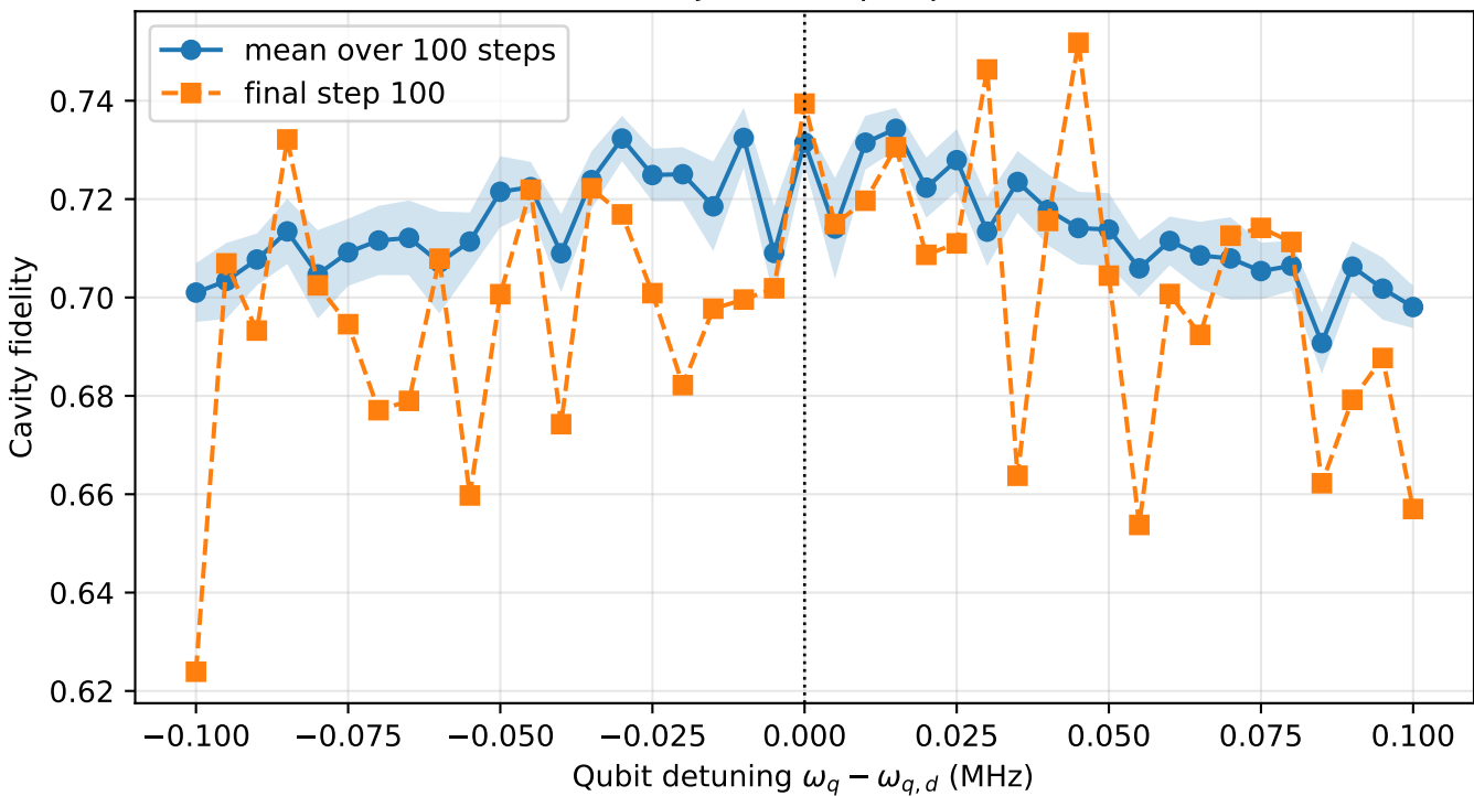
Post-training sensitivity to qubit-frequency drift 50 trajectories per point
