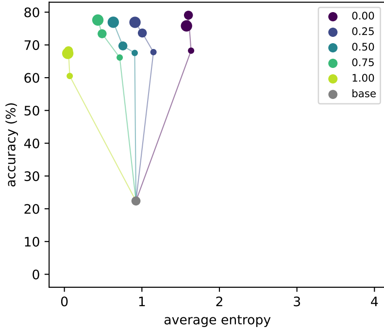
generalized JS weight (0 forward, 1 reverse)
