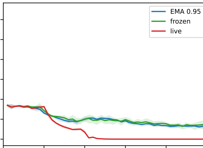
teacher
