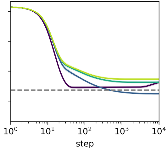
teacher top-k, tail bucket
