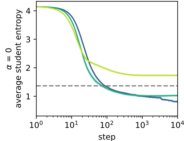
student top-k, renormalized
