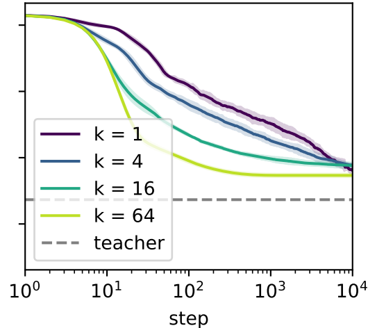
student top-k, tail bucket
