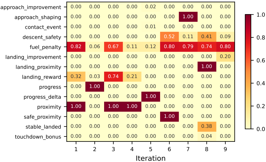
(b) Component Activation Rate
