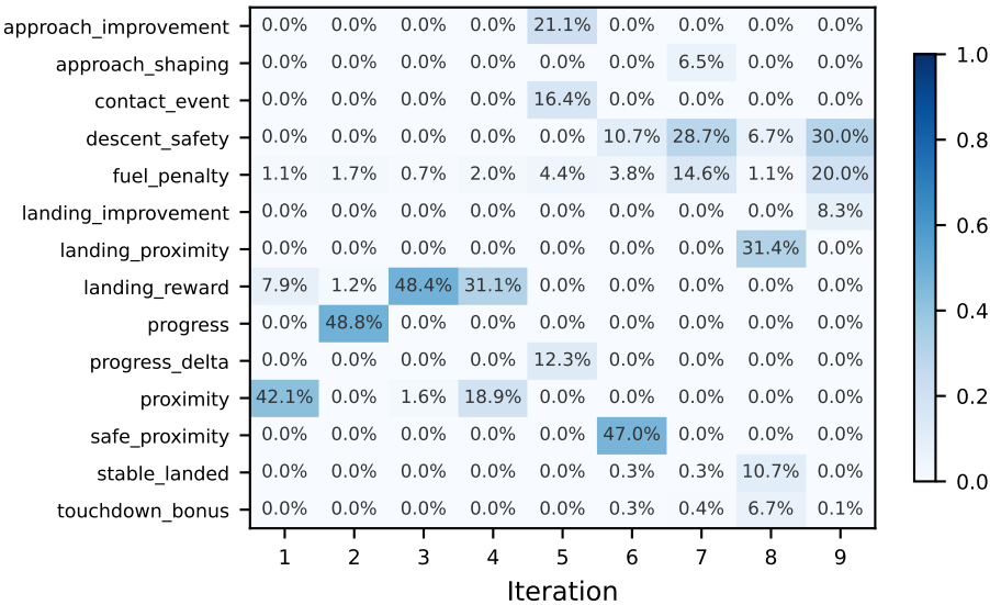
(c) Component Magnitude Share
