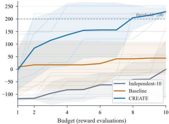
Best-so-far search fitness
