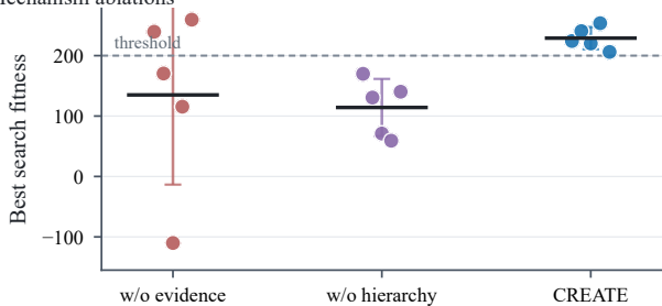
(b) Mechanism ablations
