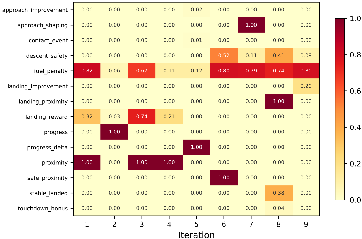
Component Activation Rate (seed 0)
