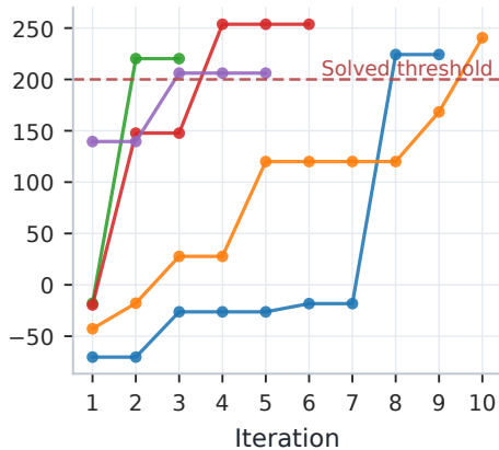
Best-so-far scores
