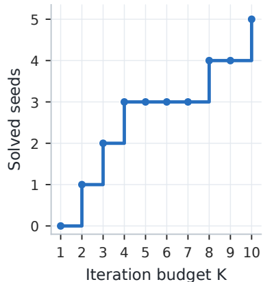
Success@K
