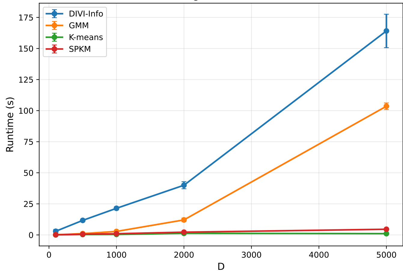
Runtime scaling with D (fixed N = 1000)
