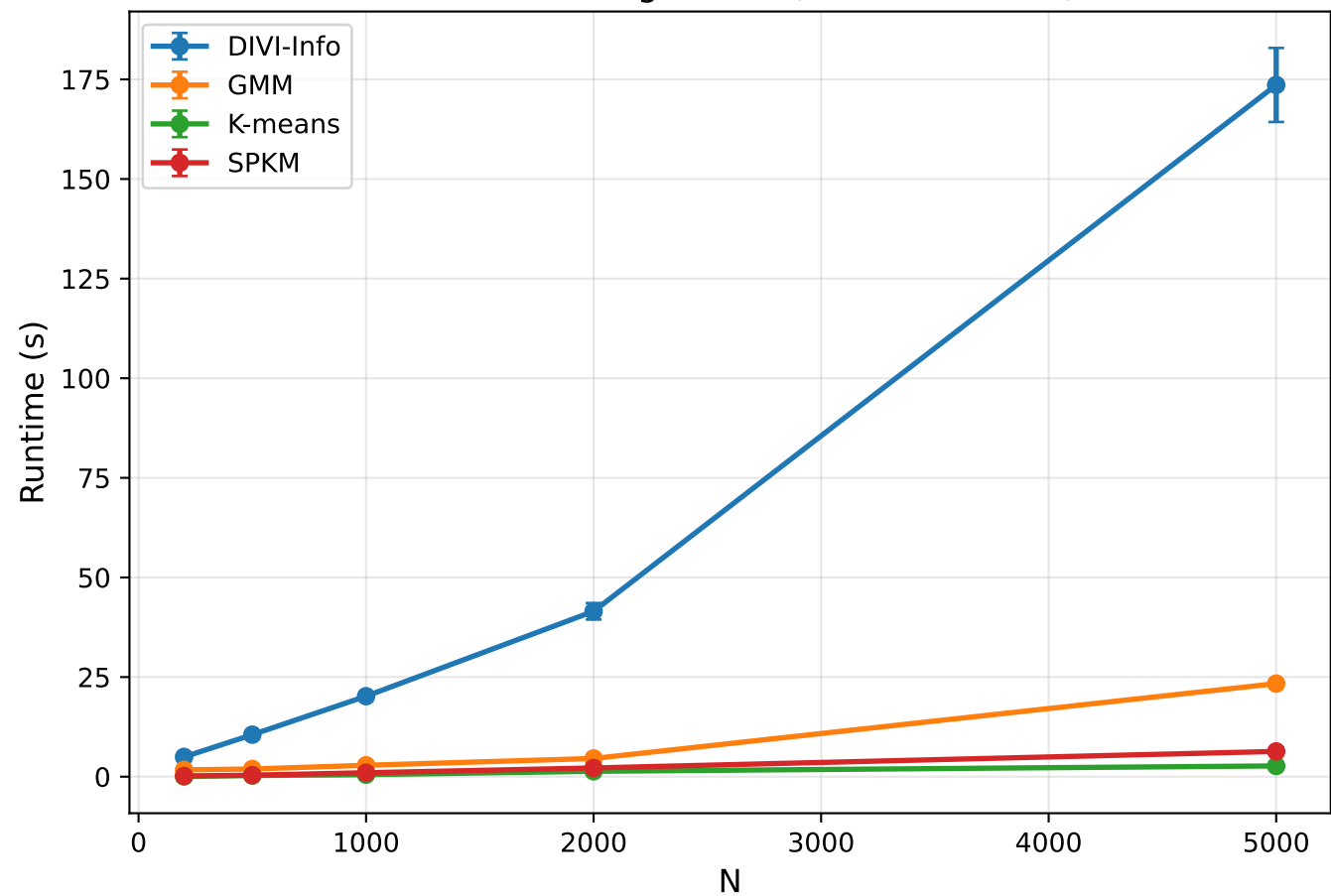
Runtime scaling with N (fixed D = 1000)
