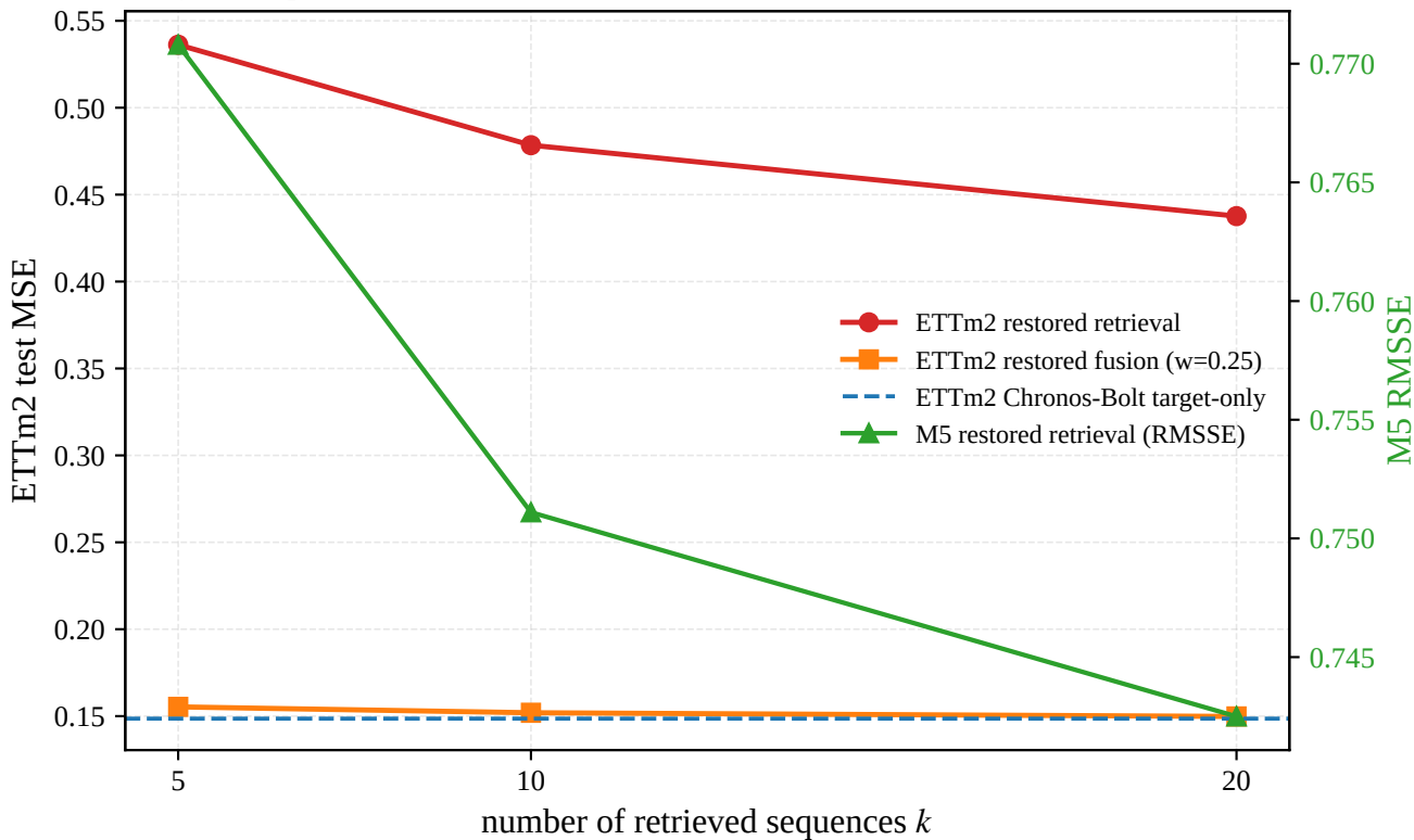
Larger k improves retrieval but fusion stays above the backbone
