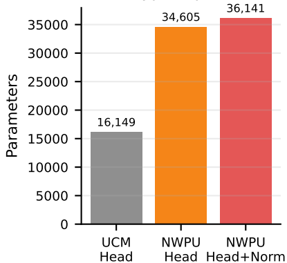
Encrypted params
