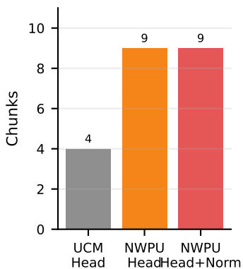
CKKS chunks
