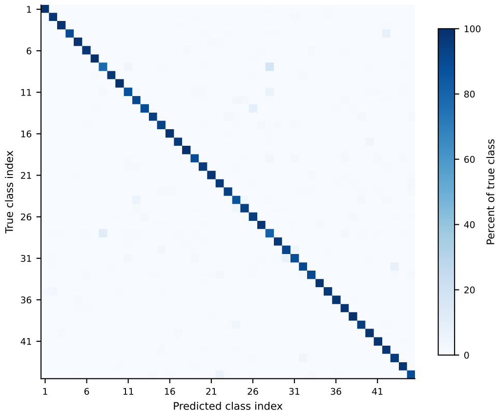
N4D01HN confusion matrix (row-normalized, seed 42)
