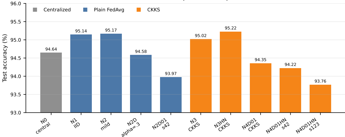
NWPU-RESISC45 experiment comparison
