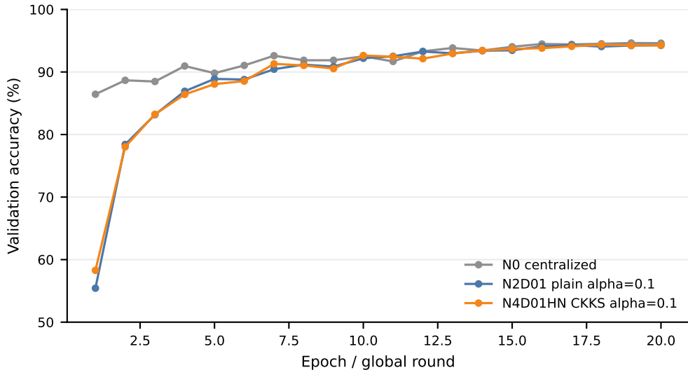
Selected validation curves
