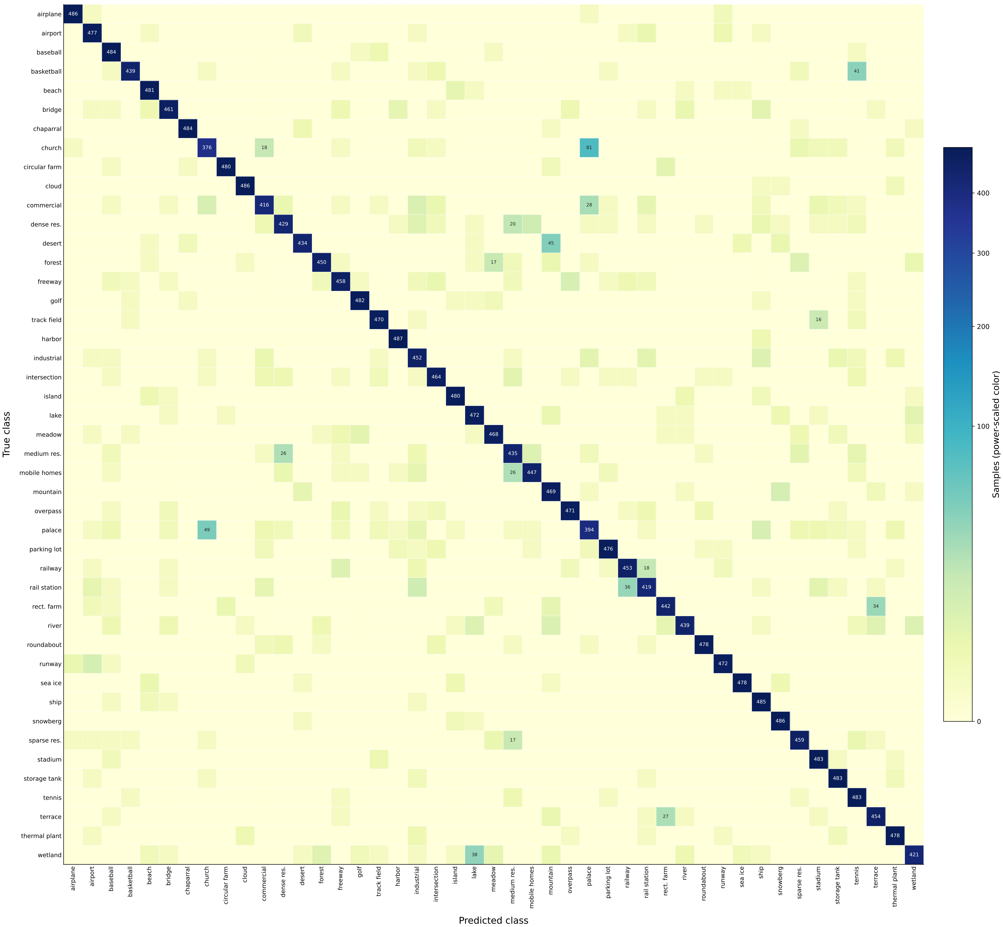
N2D01 confusion matrix (counts)
