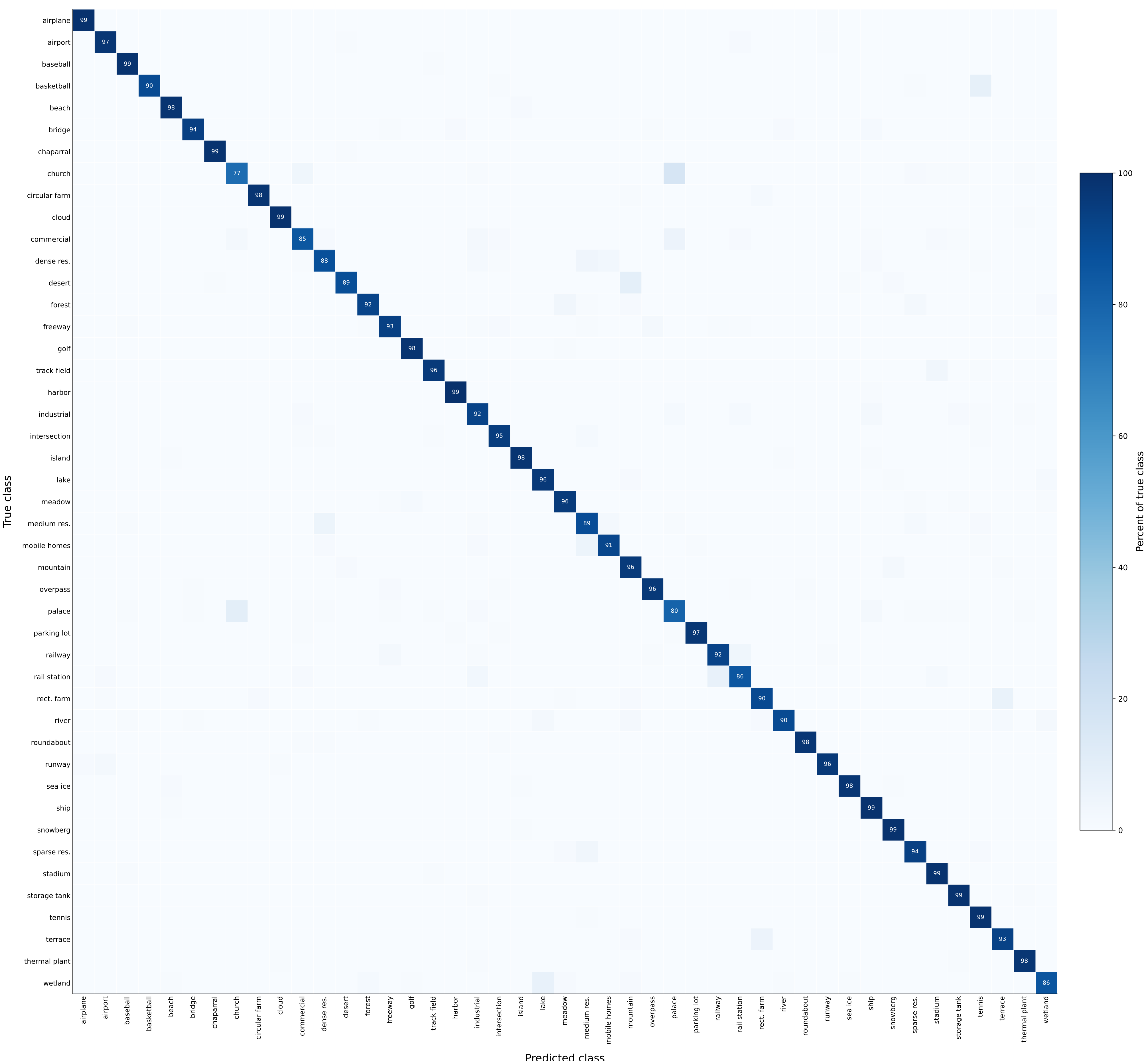
N2D01 confusion matrix (row-normalized)
