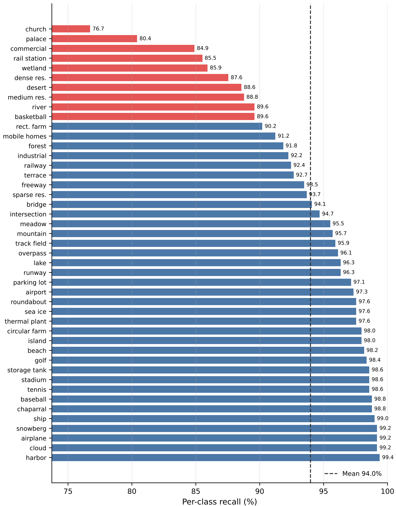
Per-class recall for N2D01
