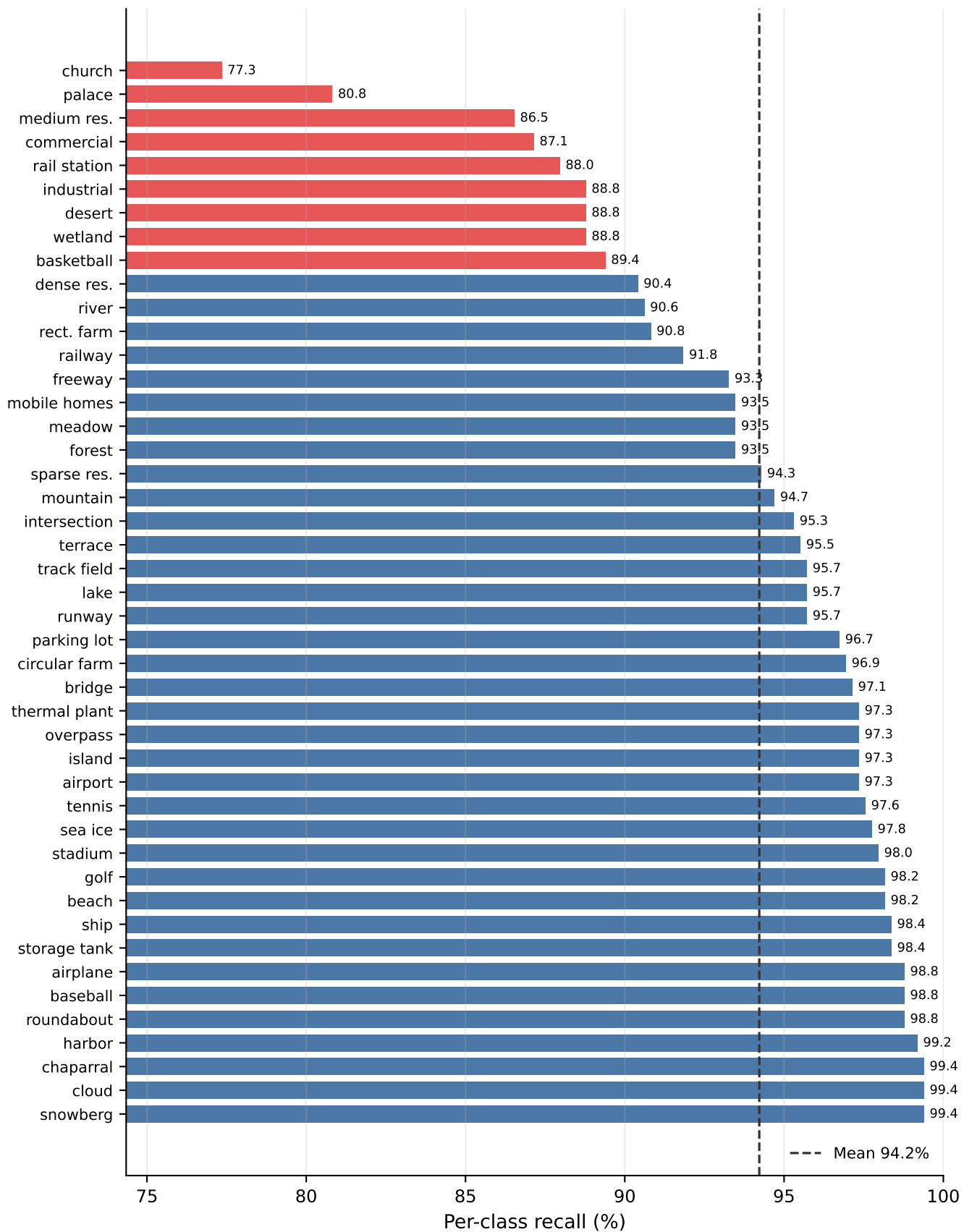
Per-class recall for N4D01HN
