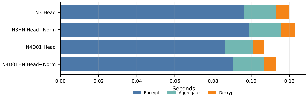
Average CKKS time per round
