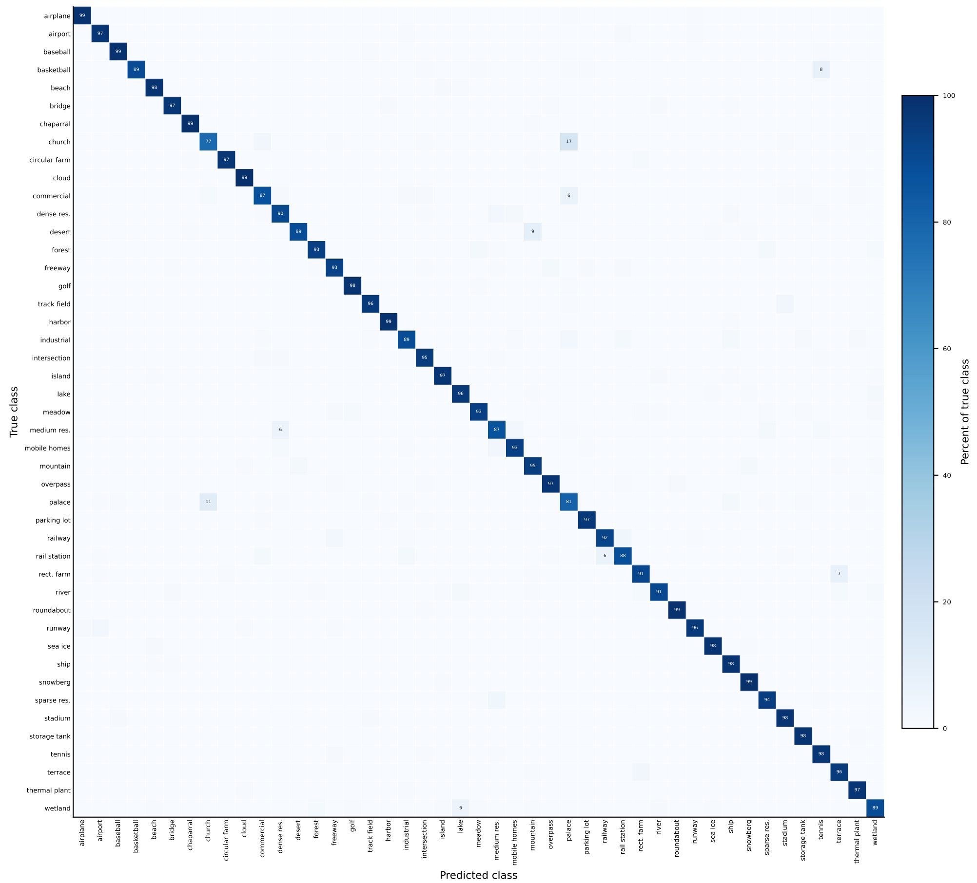
N4D01HN confusion matrix (row-normalized)
