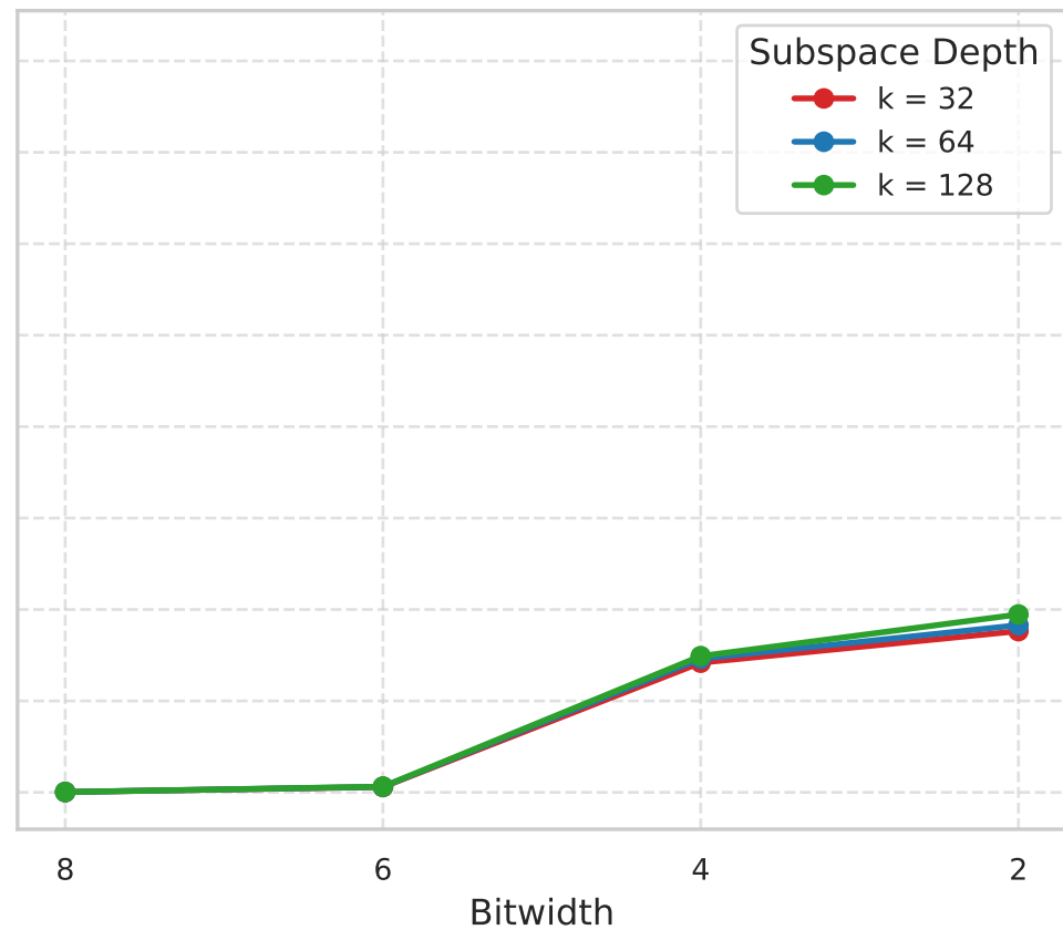
Per-Feature Quantization
