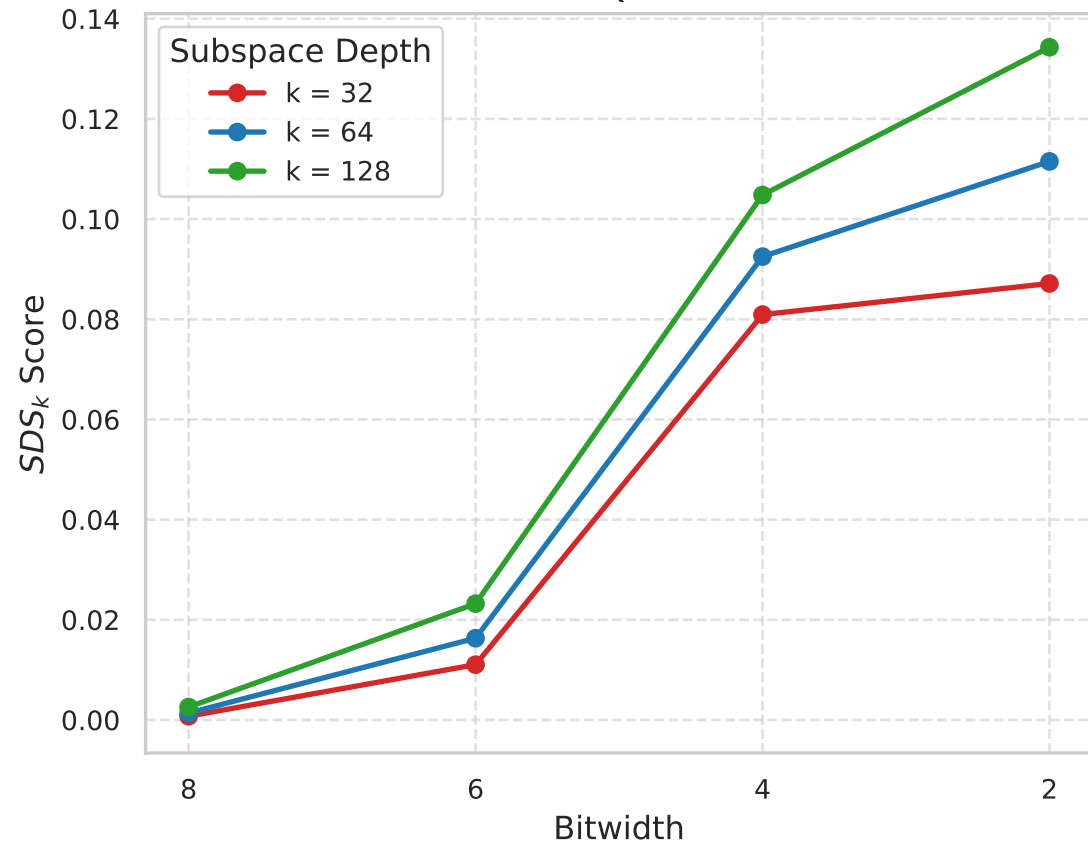
Per-Tensor Quantization
