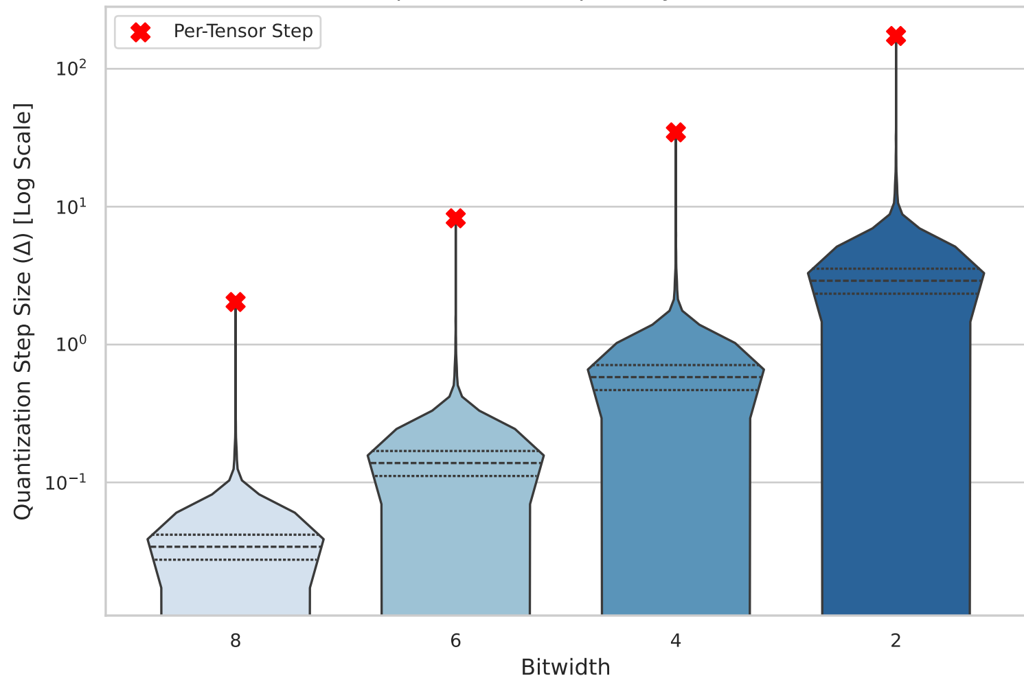
Quantization Step Size Grid Adaptability (Bottleneck m = 512 )
