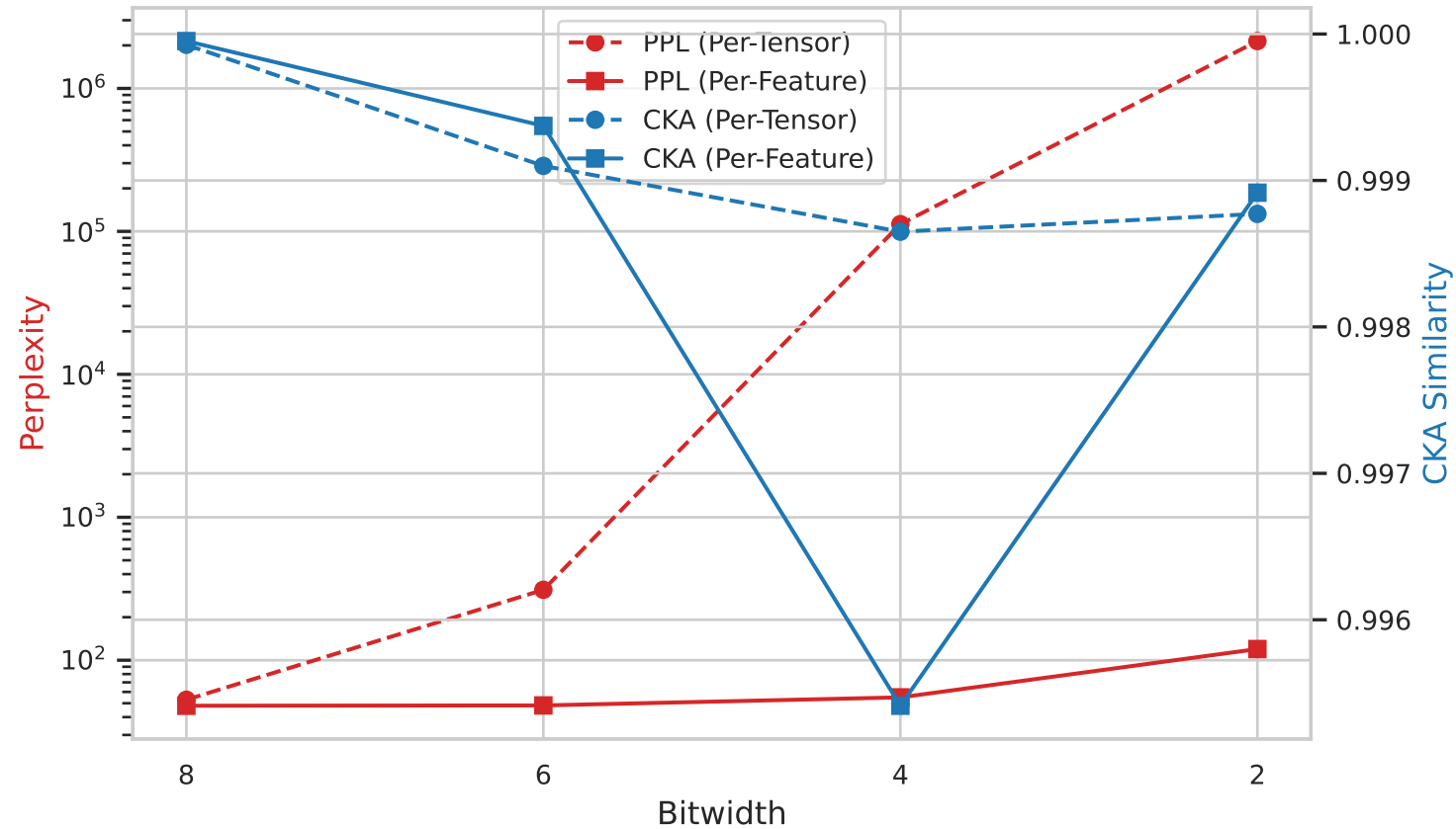
Perplexity vs. Representation CKA Alignment (Bottleneck m = 1024 )
