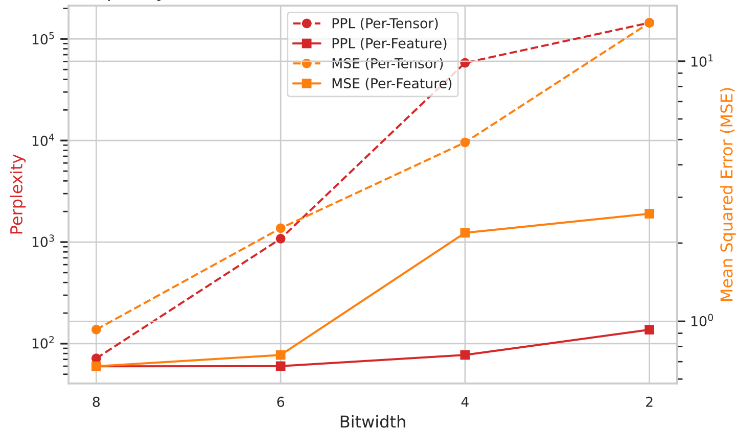
Perplexity vs. Activation Reconstruction MSE (Bottleneck m = 512 )
