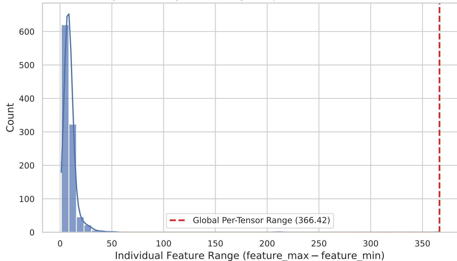
Dictionary Feature Dynamic Range Dispersion (Bottleneck m = 1024 )
